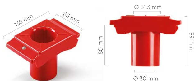
TOOL HOLDER 2"
