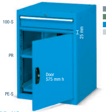
ORD. NO. DRAWERS F DD 1270 51 04 1 Cabinet with 1 normal extension drawer 1 adjustable shelf, 1 normal retractable shelf Dim. mm 564x726x800 h Central lock
