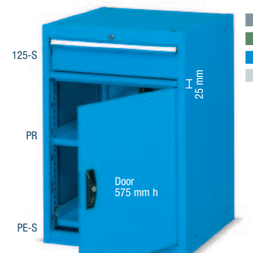
ORD. NO. DRAWERS F DD 1272 51 04 1 Cabinet with 1 normal extension drawer 1 adjustable shelf, 1 normal retractable shelf Dim. mm 564x726x825 h Central lock
