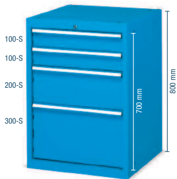
ORD. NO. DRAWERS F DD 1070 55 04 4 Cabinet with 4 normal extension drawers Dim. mm 564x726x800 h Central lock
