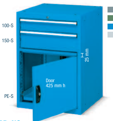
ORD. NO. DRAWERS F DD 1170 51 04 2 Cabinet with 2 normal extension drawers 1 normal retractable shelf Dim. mm 564x726x800 h Central lock
